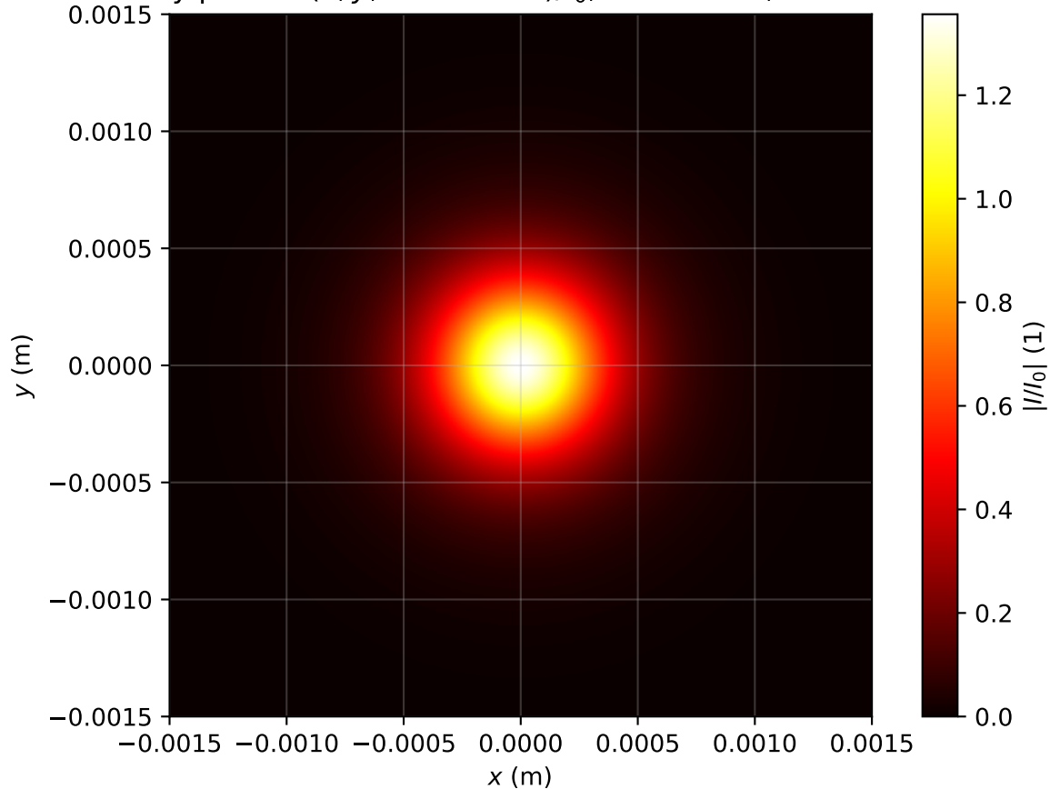
Intensity profile I(x, y, z = 1.592m)/I_0 , Pin=0.8Pcr, artificial time
